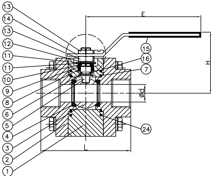
DIMENSION
